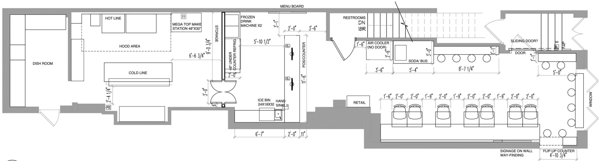
2 PRELIMINARY LAYOUT 3/16"=1'-0"
